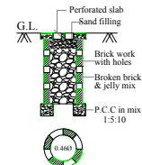
PERCOLATION PIT (NOT FOR SCALE)
