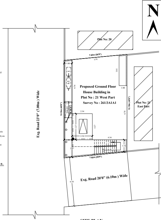
SITE PLAN
