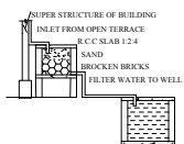
Rainwater harvesting
