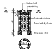
PERCOLATION PIT FOR 30 Sq. m. (Scale:- 1:50)
