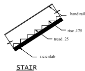
STAIR
