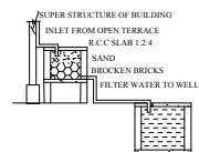
Rainwater harvesting
