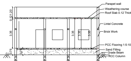
SECTION ON - X - X
