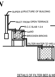
DETAILS OF FILTER BED & WELL NTS
