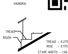
STAIRCASE DETAILS NTS
