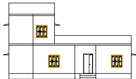
FRONT ELEVATION
