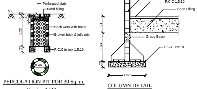
PERCOLATION PIT FOR 30 Sq. m. (Scale:- 1:50)
