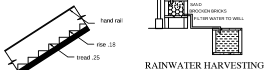
RAINWATER HARVESTING
