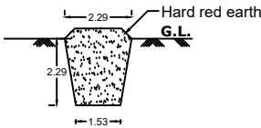
TRIAL PIT (Scale 1:100)
