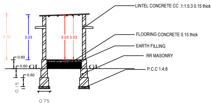
SECTION "A-B"
