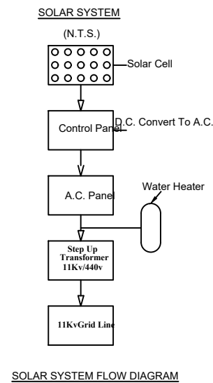
SOLAR SYSTEM FLOW DIAGRAM
