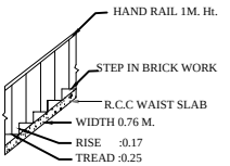
STAIR DETAIL
