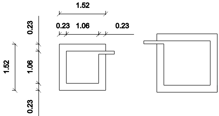
DETAILS OF FILTER BED & WELL
