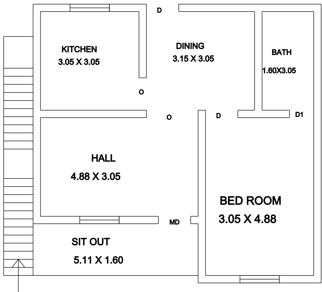
EXT.GROUND FLOOR PLAN
