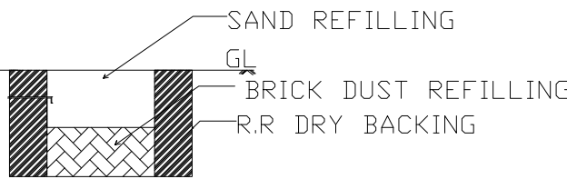
DETAILS OF RAIN WATER HARVESTING
