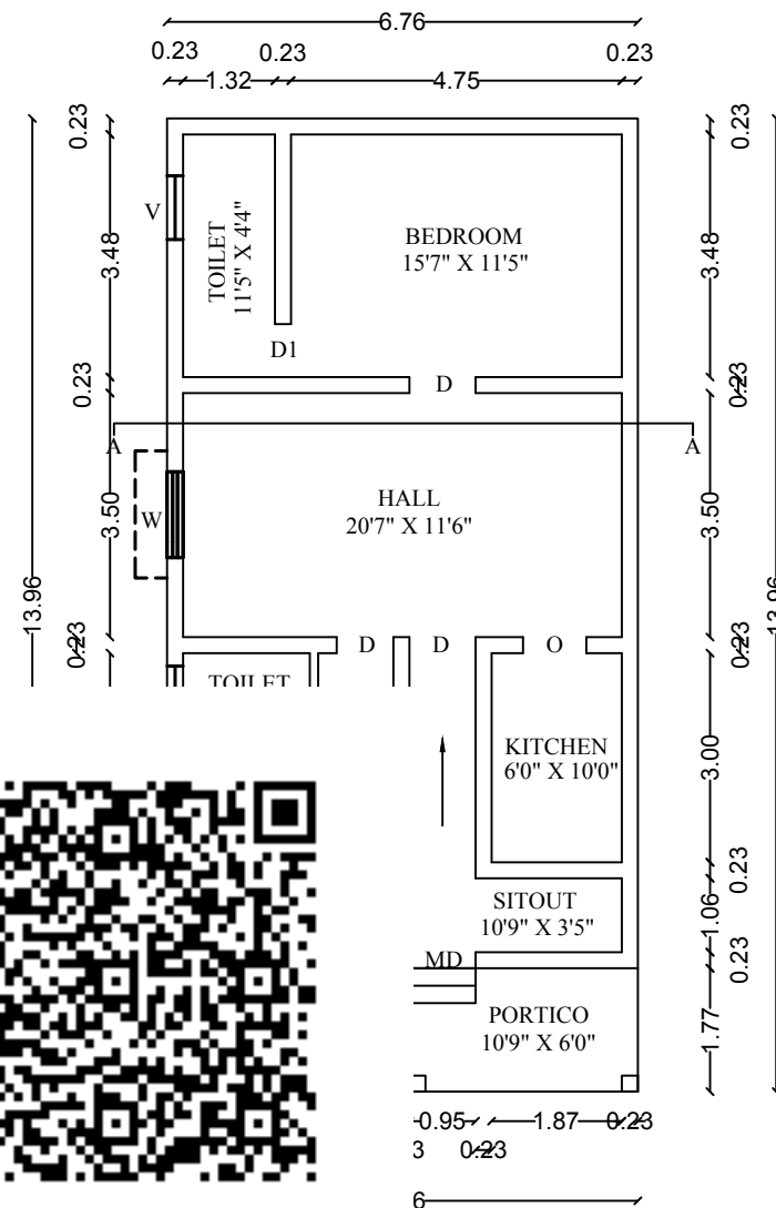
FLOOR PLAN
