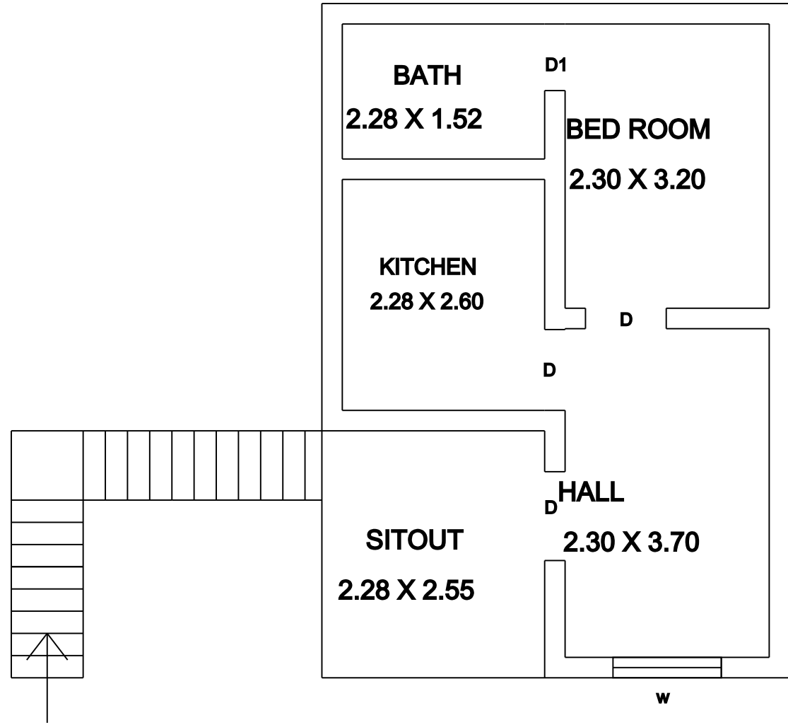
EXT.GROUND FLOOR PLAN
