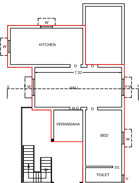
FIRST FLOOR PLAN [pro]
