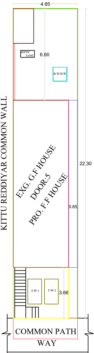
SITE PLAN
