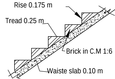
STAIR DETAILS
