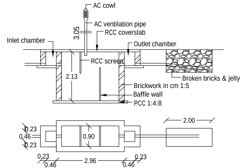
SEPTICTANK DETAILS
