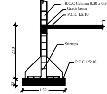
Column Detail
