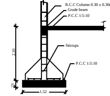
Column Detail
