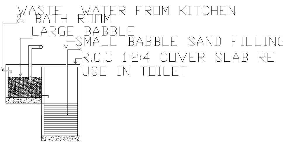
RECYCLING OF WASTE WATER FROM KITCHEN & BATHROOM
