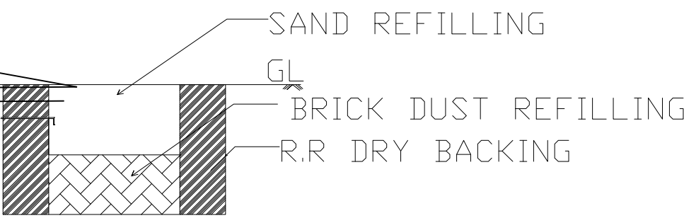
DETAILS OF RAIN WATER HARVESTING
