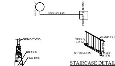
STAIRCASE DETAILS
