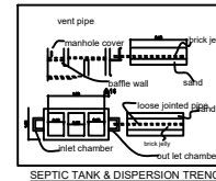
SEPTIC TANK & DISPERSION TRENCH
