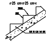
STAIRCASE DETAILS
