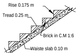
STAIR DETAILS
