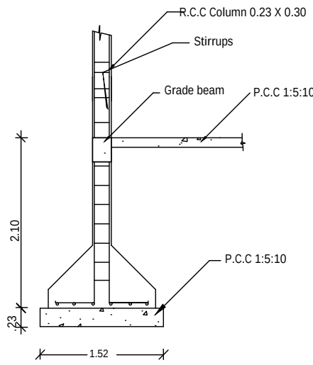
COLUMN DETAIL
