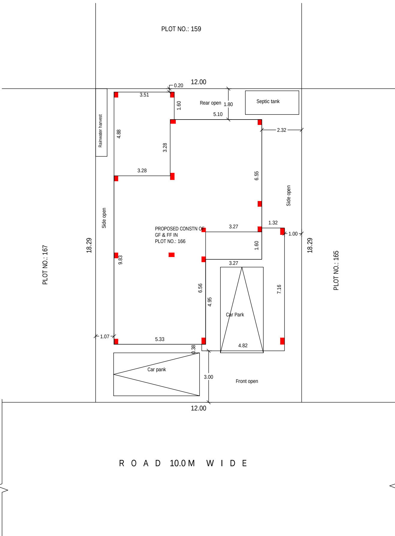
SITE PLAN
