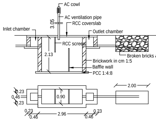
SEPTICTANK DETAILS
