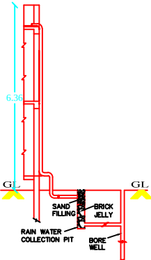
RAIN WATER HARVESTING SYSTEM
