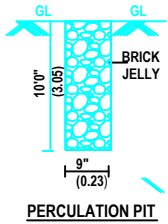
PERCOLATION PIT
