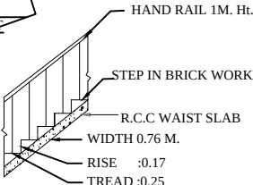
STAIR DETAIL
