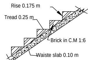
STAIR DETAILS
