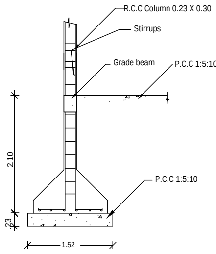
COLUMN DETAIL
