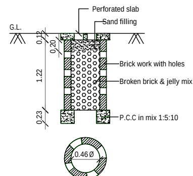
PERCOLATION PIT FOR 30 Sq. m. (Scale:- 1:50)
