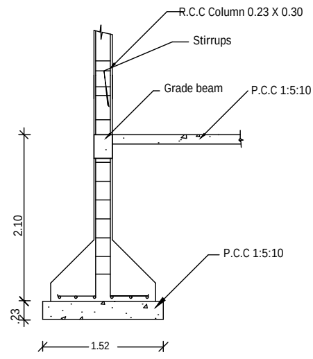
COLUMN DETAIL
