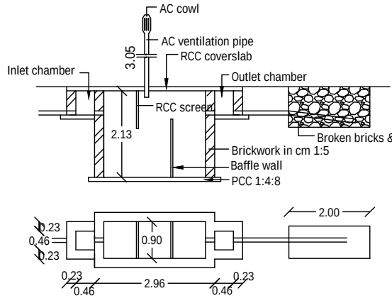
SEPTICTANK DETAILS
