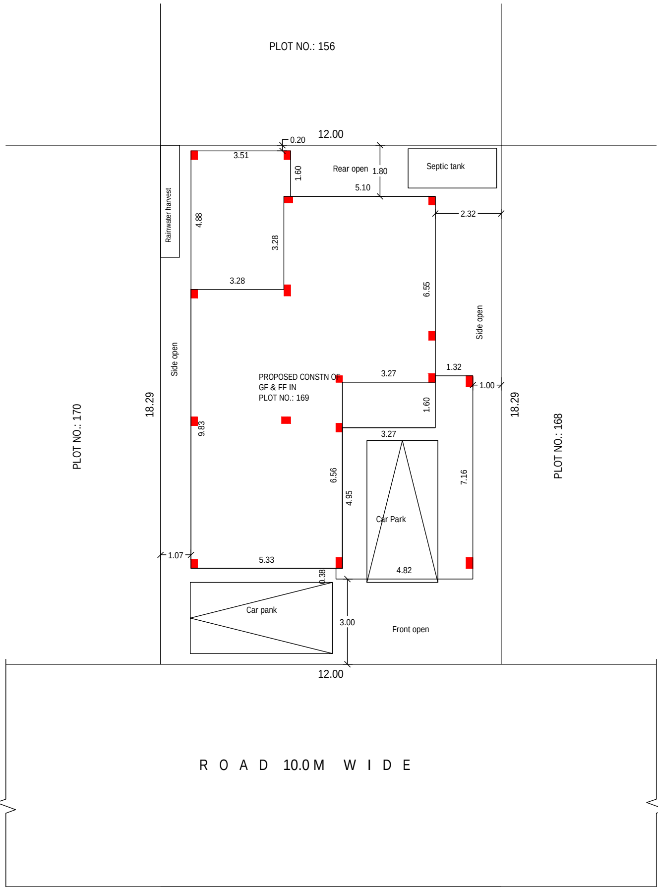
SITE PLAN
