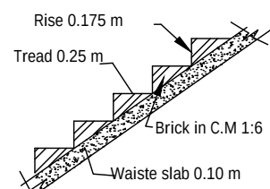
STAIR DETAILS
