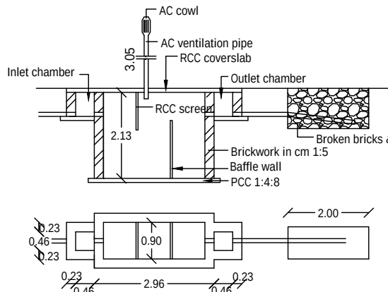
SEPTICTANK DETAILS
