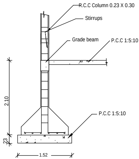
COLUMN DETAIL
