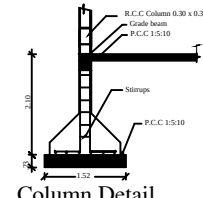
Column Detail
