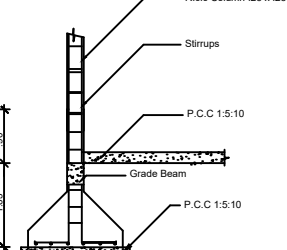
COLUMN DETAIL
