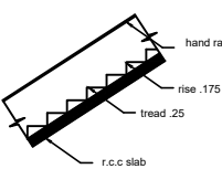
STAIR
