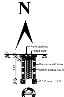
PERCOLATION PIT FOR 30 Sq. m. (Scale:- 1:50)
