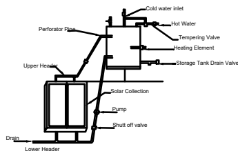
Details of Solar Water Heater (NTS)
