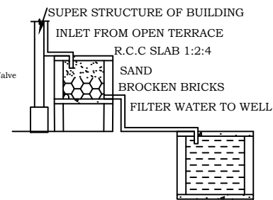
RAINWATER HARVESTING
