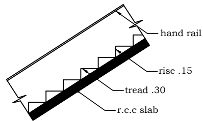
STAIR
