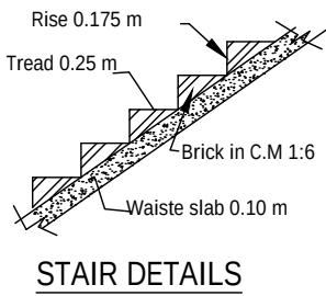
STAIR DETAILS
