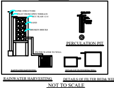
RAINWATER HARVESTING
