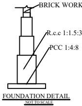
FOUNDATION DETAIL
