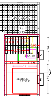
FLOOR PLAN
