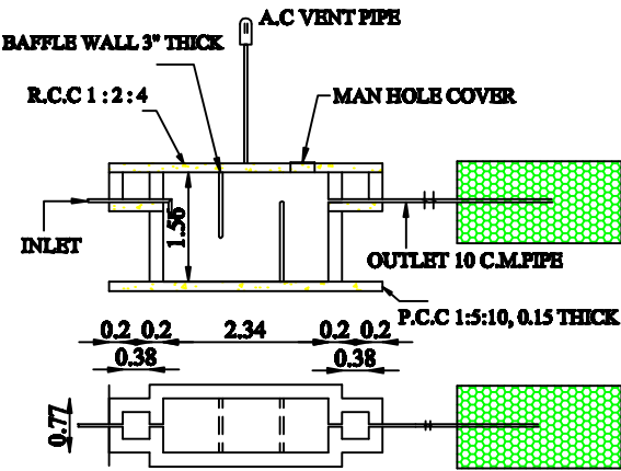
SEPTIC TANK AND DETAILS
