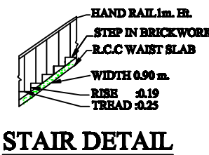
STAIR DETAIL
