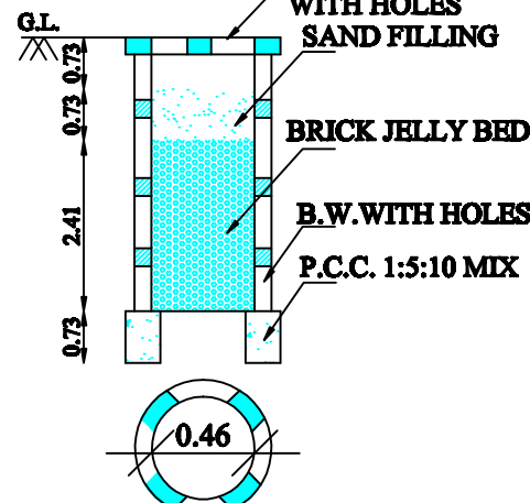
PERCOLATION PIT
