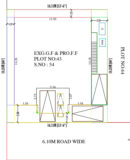
SITE PLAN(1:100)
