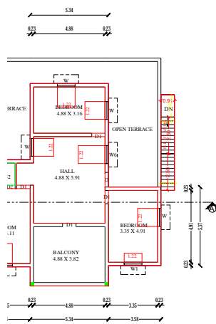
PRO-FIRST FLOOR PLAN
