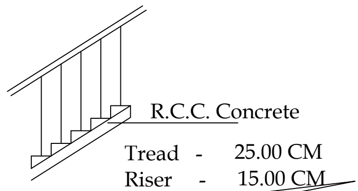
Staircase details
