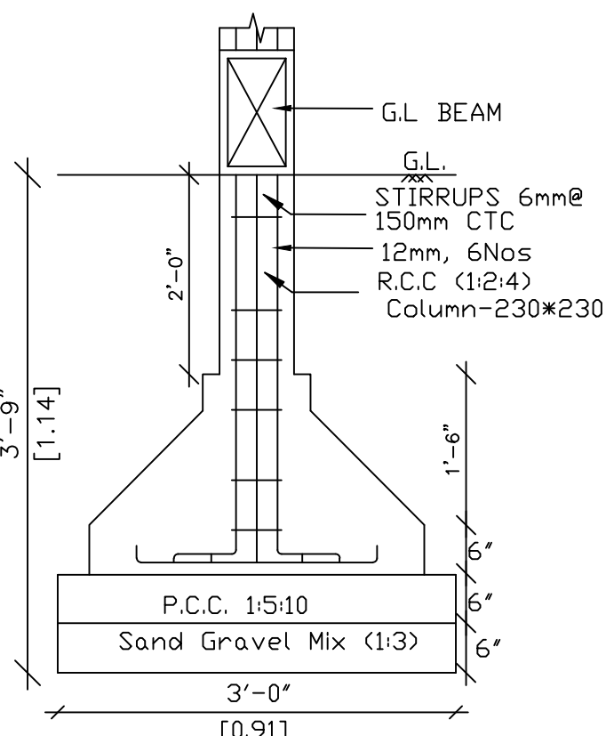
R.C.C. COLUMN FOOTING DETAILS
