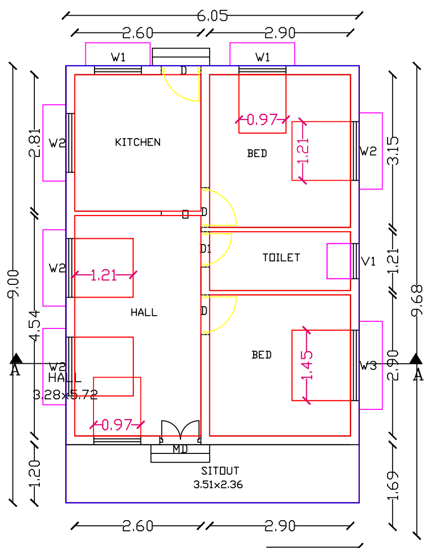
PLAN
