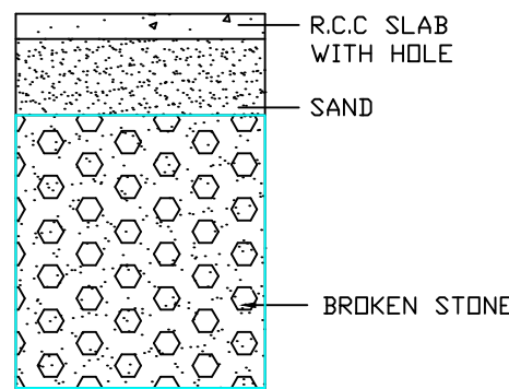
RAIN WATER HARVEST COLLECTION PIT.
