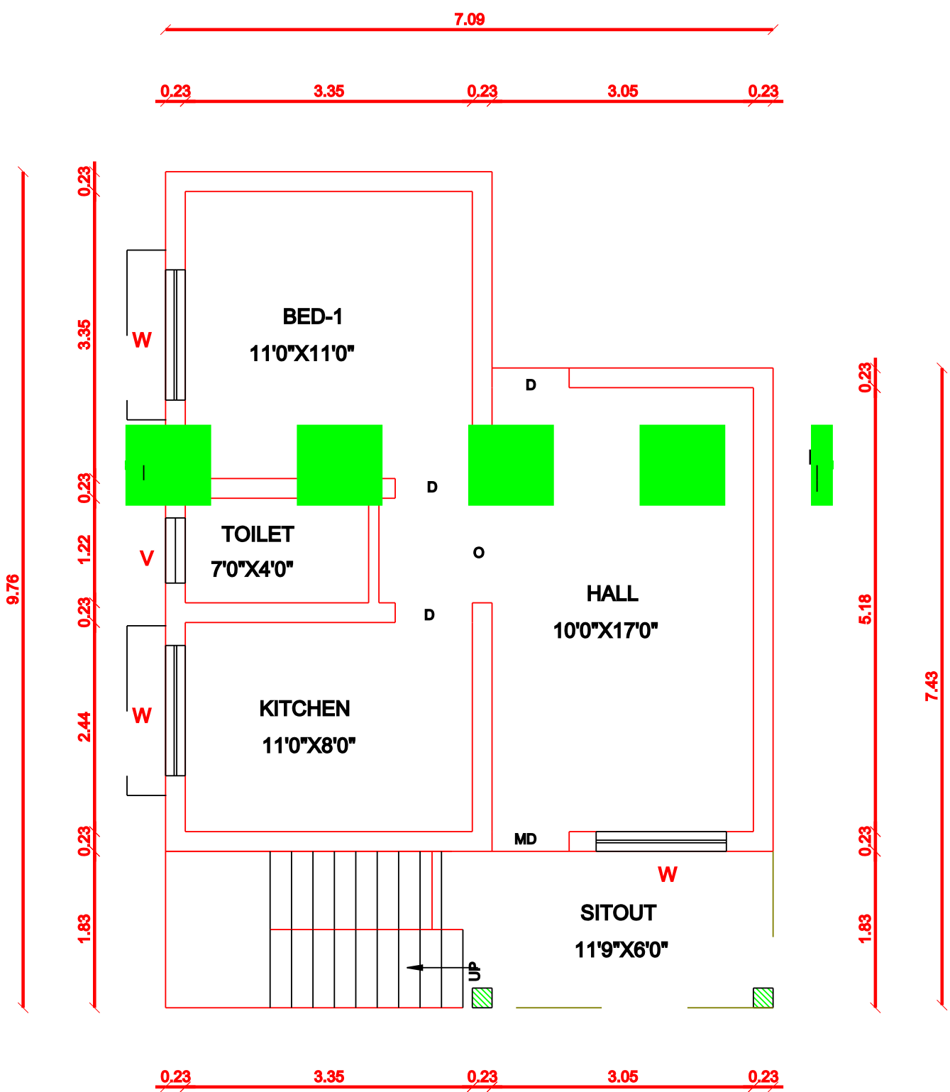
FLOOR PLAN
