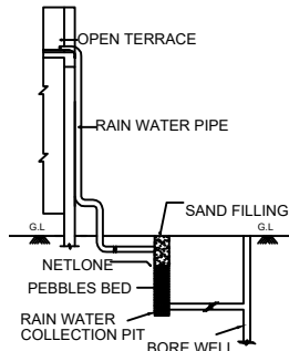
RAIN WATER VESTING SYSTEM
