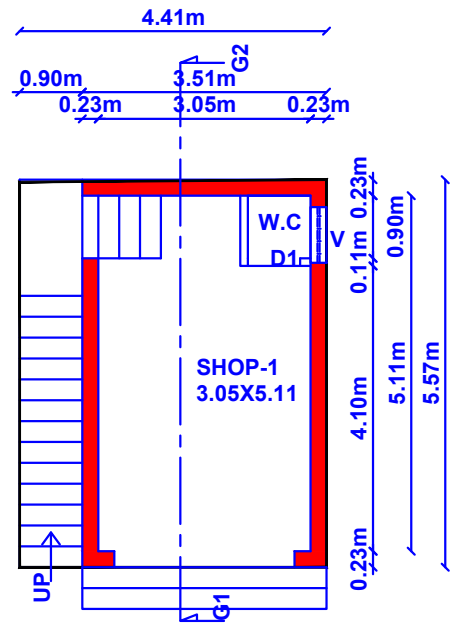
GROUND FLOOR PLAN (Dronead)
