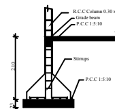
Column Detail
