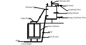
Details Of Solar Water Heater (NTS)
