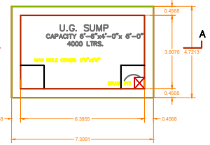
SUMP DETAIL
