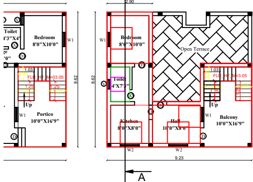
EXG.GROUND FLOOR PLAN
