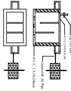
Septic Tank and Trench
