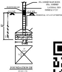
FOUNDATION DETAIL
