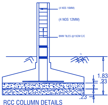
RCC COLUMN DETAILS
