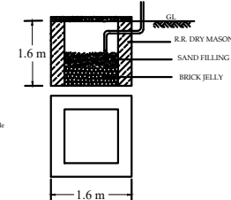
RAINWATER HARVESTING DETAILS
