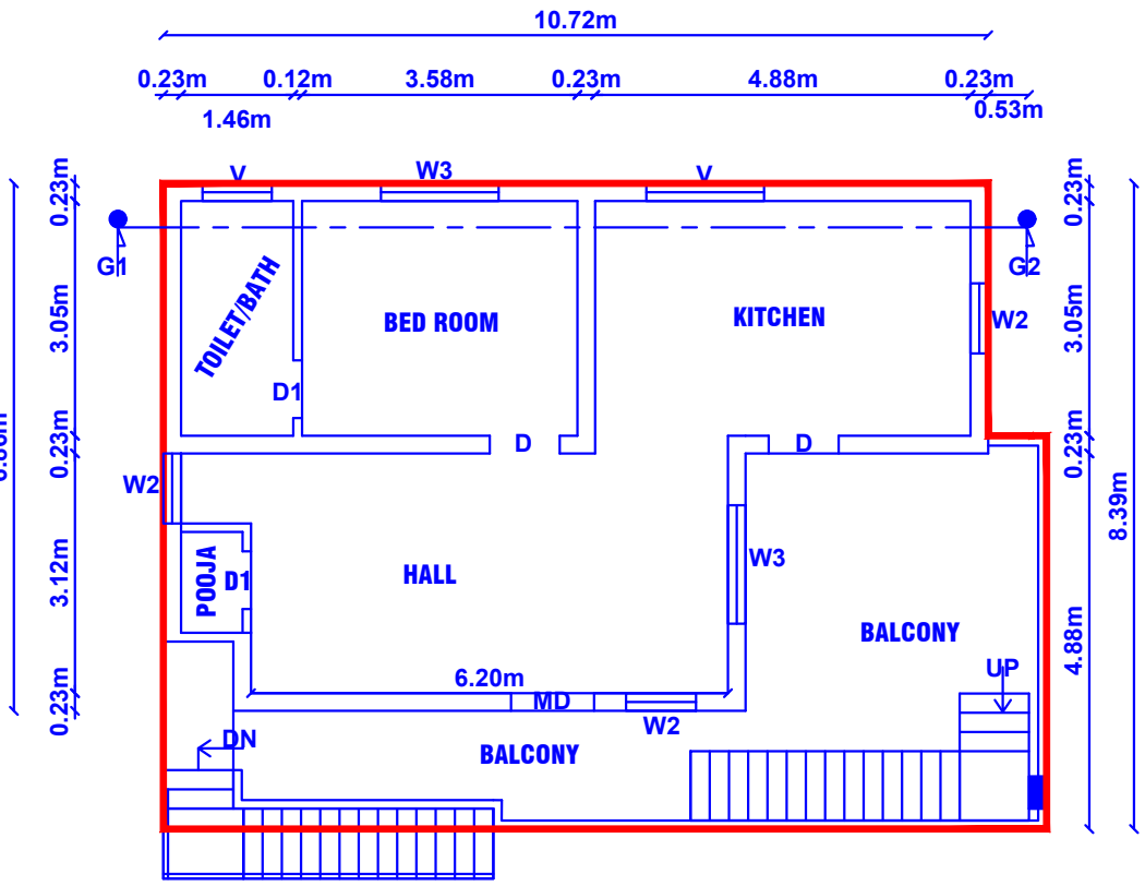
FIRST FLOOR PLAN (Proposed)
