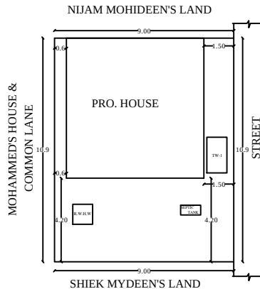
SITE PLAN
