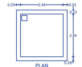
PLAN DETAILS OF COLLECTION SUMP FOR RAIN WATER HARVESTING OF ROOF TOP RAIN WATER
