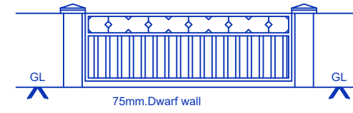
COMPOUND WALL/ ENTRANCE GATE
