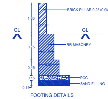
FOOTING DETAILS
