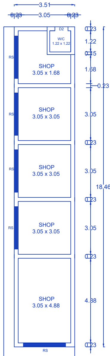
GROUND FLOOR PLAN BLOCK 2
